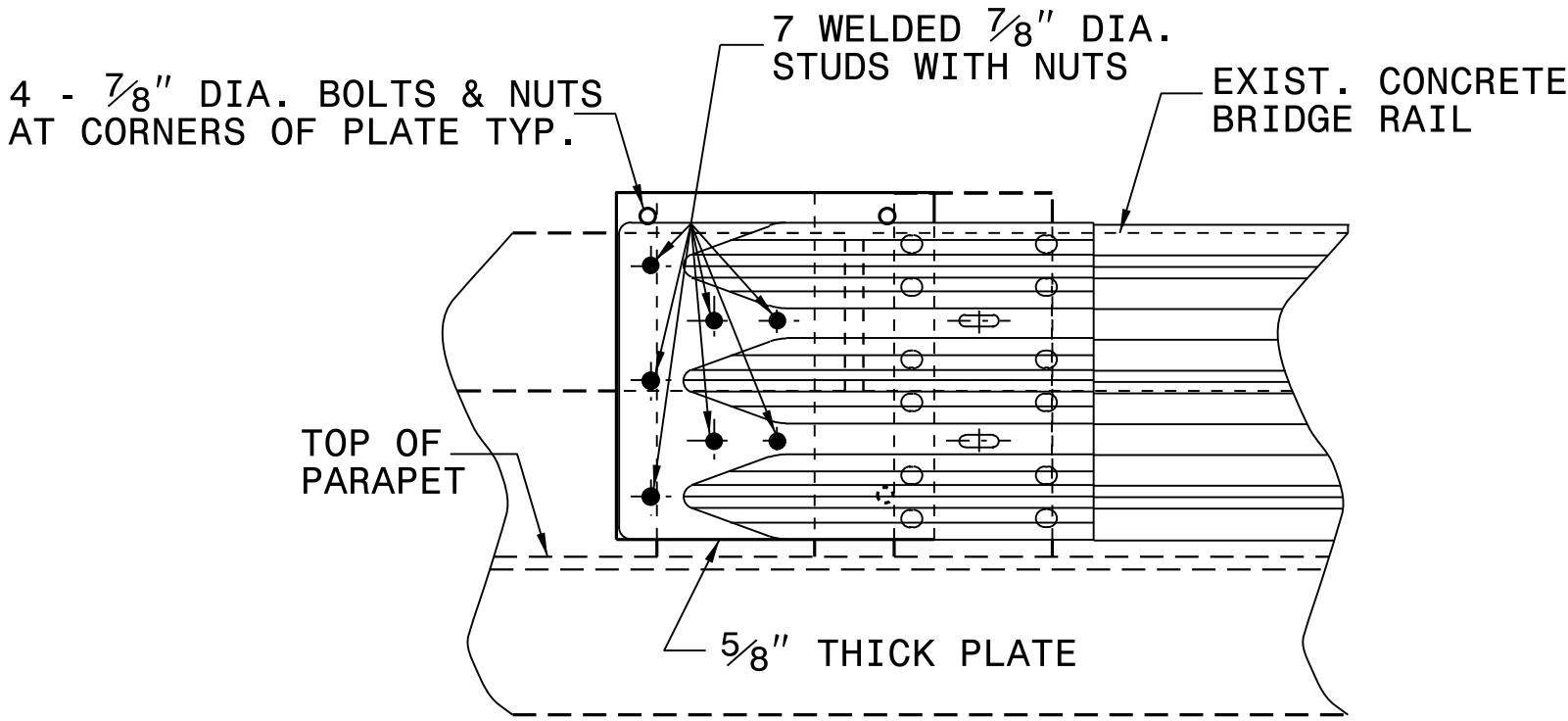
ELEVATION VIEW
