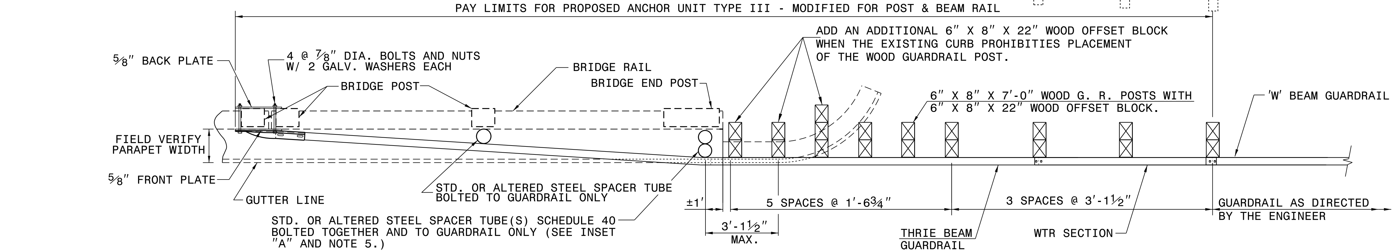
PLAN VIEW
